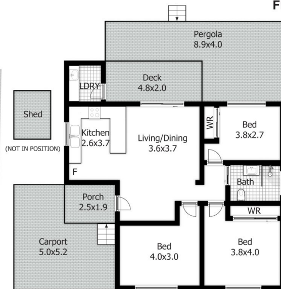
MAIN HOUSE
